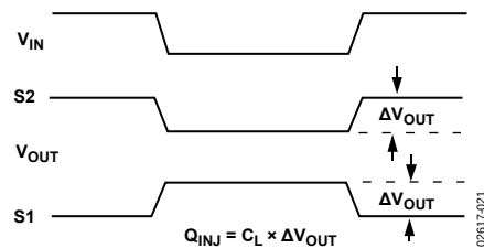
Figure 21. Charge Injection
