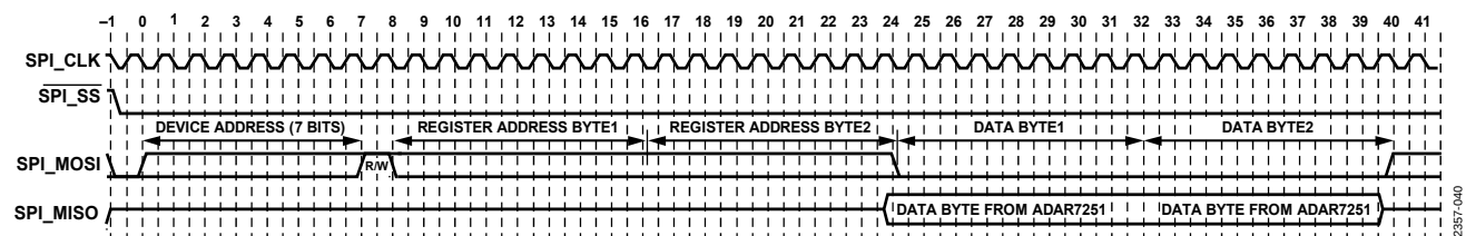
Figure 54. SPI Read from the ADAR7251 Clcking (Single-Word Read Mode), No CRC
