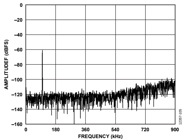
Figure 13. FFT with -60 dBFS, 100 kHz Input at f_s = 1.8 MHz
