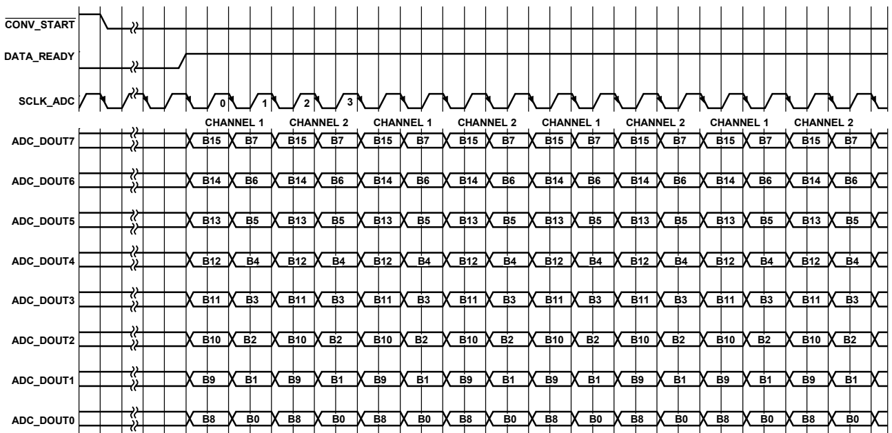
Figure 45. PPI, 2-Channel
