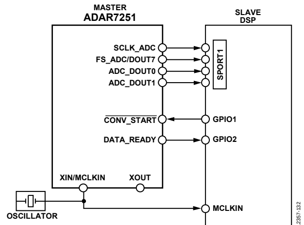
Figure 40. ADC Serial Master Mode with CONV_START
