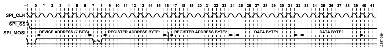
Figure 53. SPI Write to the ADAR7251 Clcking (Single-Word Write Mode), No CRC
