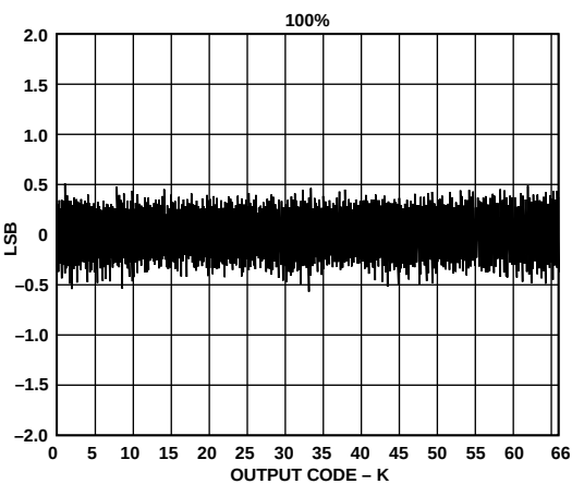
Figure 12. DNL Plot
