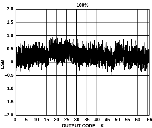
Figure 11. INL Plot
