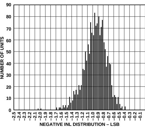
Figure 16. Typical Negative INL Distribution (1516 Units)
