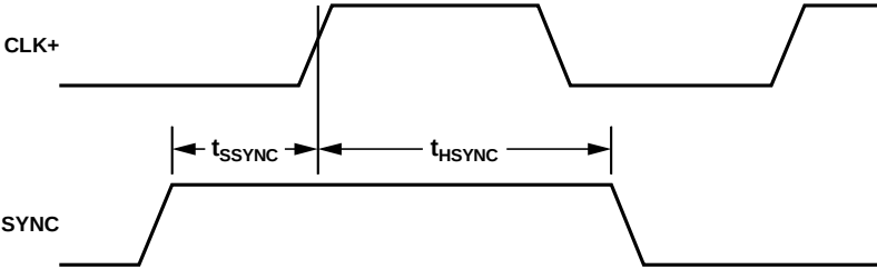
Figure 5. SYNC Input Timing Requirements
