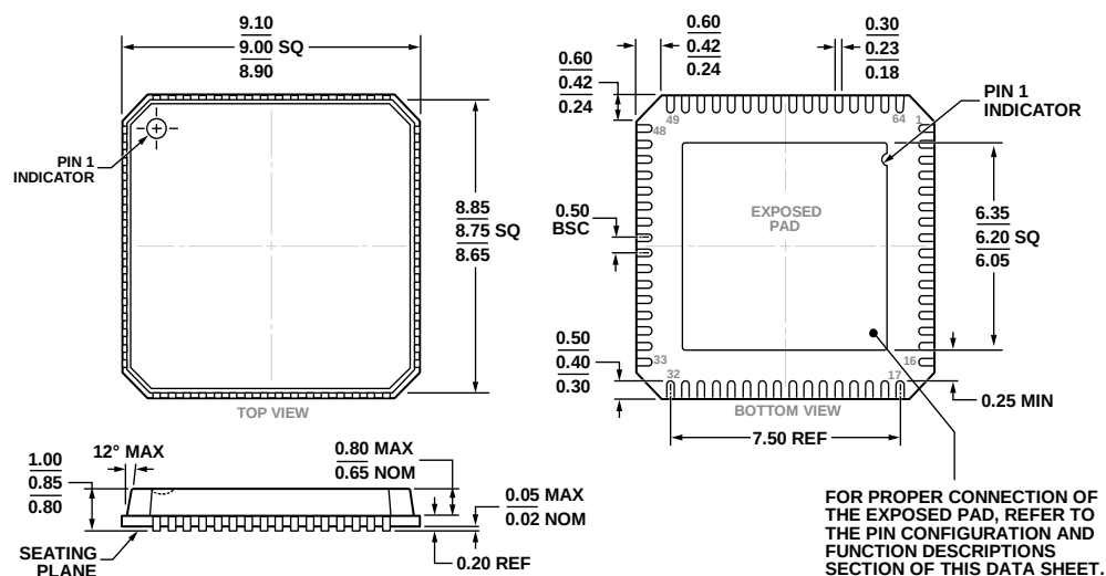
Figure 62. 64-Lead Lead Frame Chip Scale Package [LFCSP_VQ] 9 mm × 9 mm Body, Very Thin Quad (CP-64-4)
