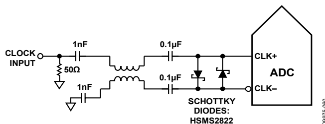
Figure 53. Balun-Coupled Differential Clock (Up to 1 GHz)
