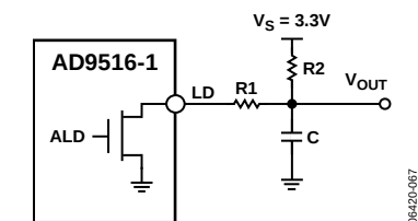
Figure 50. Example of Analog Lock Detect Filter, Using N-Channel Open-Drain Driver
