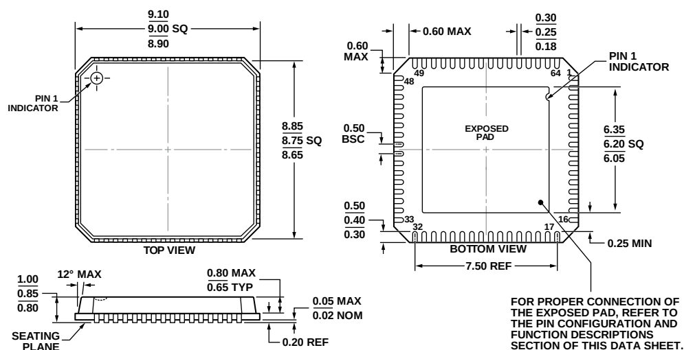
Figure 77. 64-Lead Lead Frame Chip Scale Package [LFCSP_VQ] 9 mm x 9 mm Body, Very Thin Quad CP-64-4 Dimensions shown in millimeters
