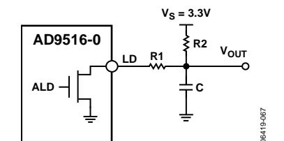
Figure 50. Example of Analog Lock Detect Filter, Using N-Channel Open-Drain Driver
