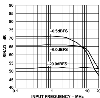
Figure 14. SINAD vs. Input Frequency (Input Span = 2 V, V_{\text{CM}} = 2.5\text{ V} )
