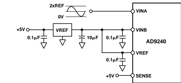
Figure 43. Input Range = 0 V to 2 \times V_{REF}
