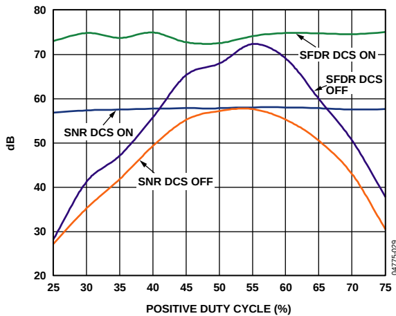
Figure 24. SNR, SFDR vs. Positive Duty Cycle DCS Enabled, Disabled; A_{IN} = 70 MHz at –0.5 dBFS, 105 MSPS (–105 Grade)
