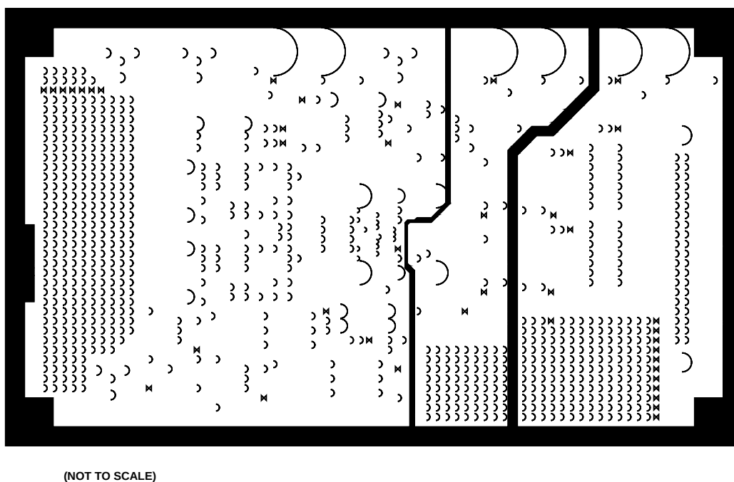
Figure 41. Evaluation Board Power Plane Layout
