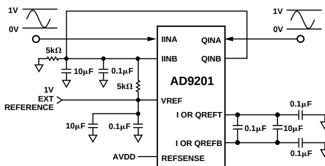
Figure 25. External Reference
