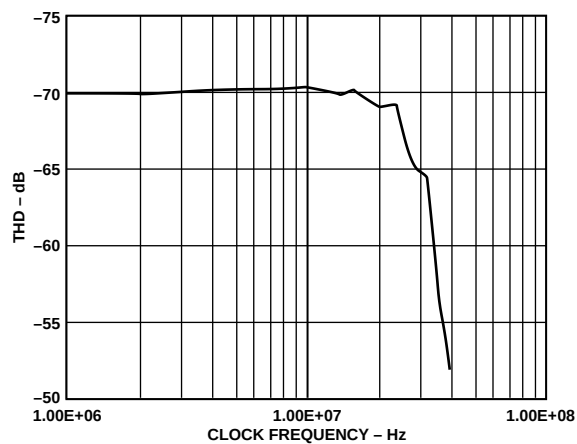
Figure 9. THD vs. Clock Frequency ( f_{IN} = 1 MHz)
