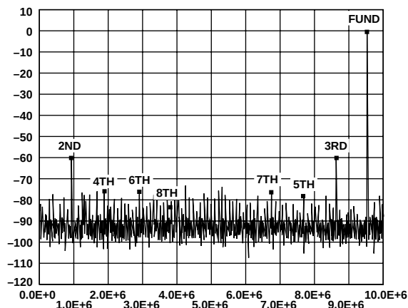
Figure 28. AD8051/AD9201 Performance
