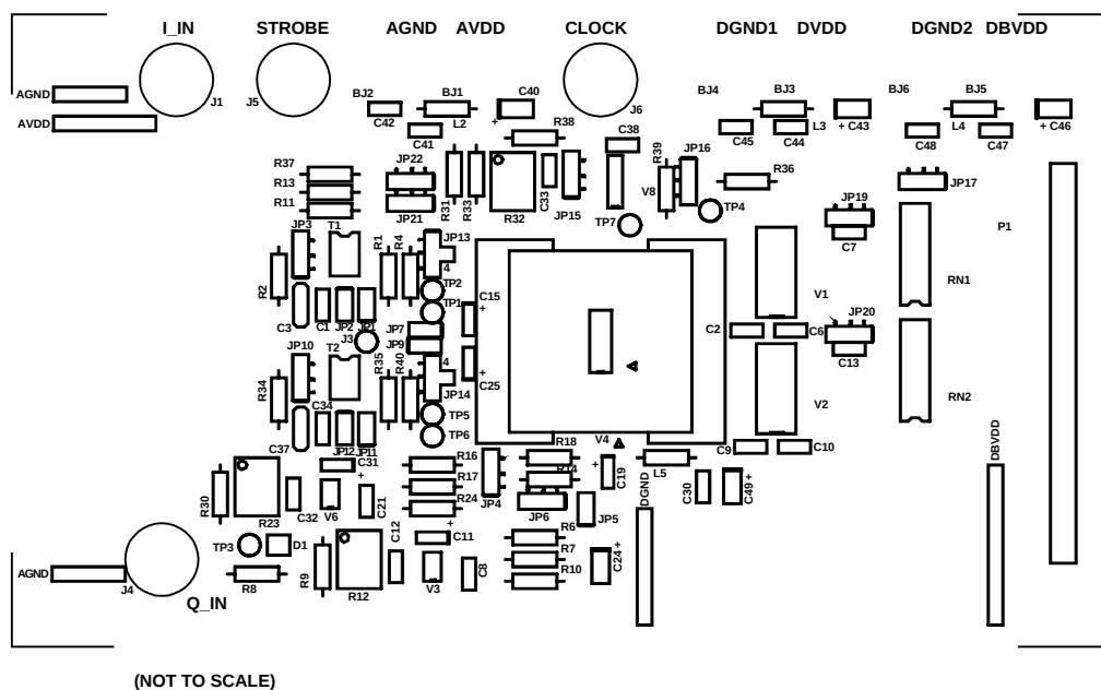
Figure 40. Evaluation Board Component-Side Silkscreen
