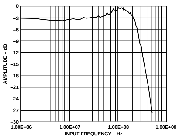
Figure 13. Full Power Bandwidth
