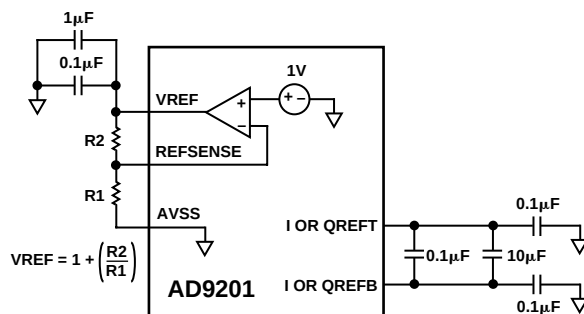
Figure 24. Programmable Reference
