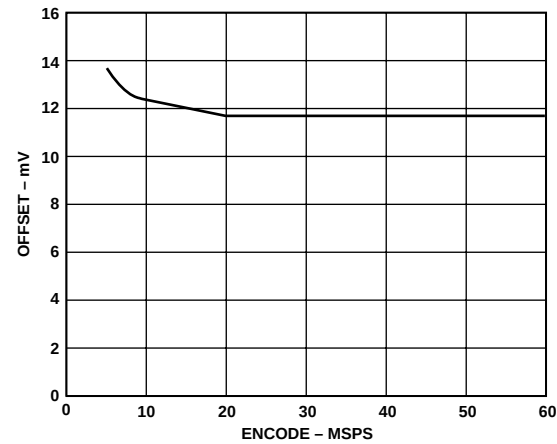
TPC 14. Offset vs. Clock Rate
