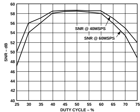
TPC 15. SNR vs. Duty Cycle
