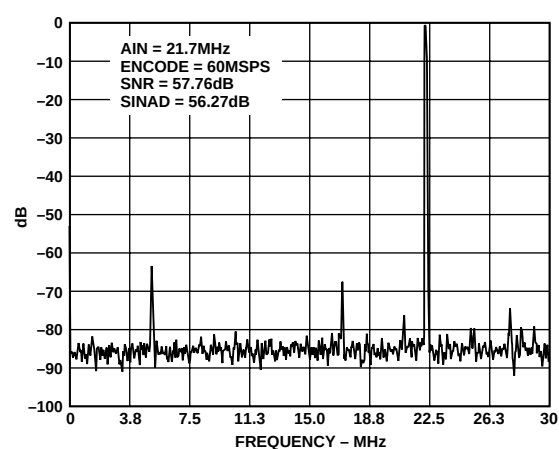
TPC 11. FFT Plot 60 MSPS, 21.7 MHz
