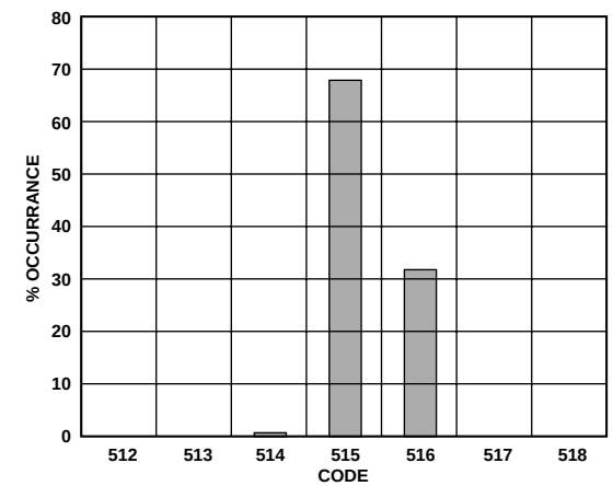
TPC 18. Midscale Histogram (Inputs Tied)
