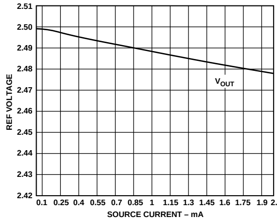
TPC 17. Reference Load Regulation
