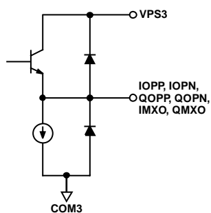
Figure 37. Circuit B
