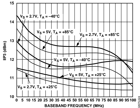
Figure 15. IIP3 vs. F_{BB} , V_{GIN} = 1.2 V, F_{LO} = 1900 MHz
