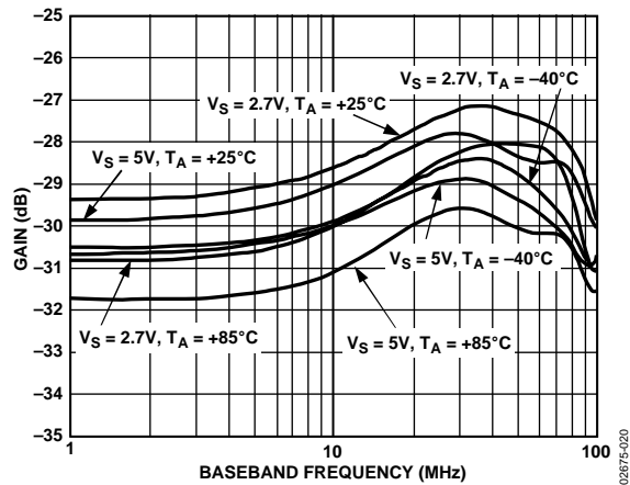
Figure 11. Gain vs. F_{BB} , V_{GIN} = 1.2 V, F_{LO} = 1900 MHz
