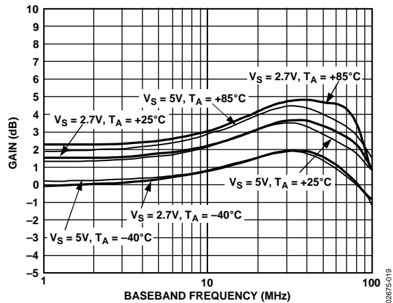
Figure 10. Gain vs. F_{BB} , V_{GIN} = 0.7 V, F_{LO} = 1900 MHz
