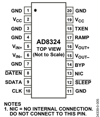
Figure 6. 20-Lead QSOP Pin Configuration
