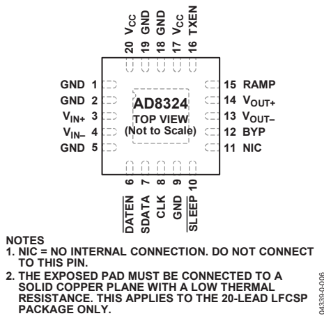
Figure 5. 20-Lead LFCSP Pin Configuration
