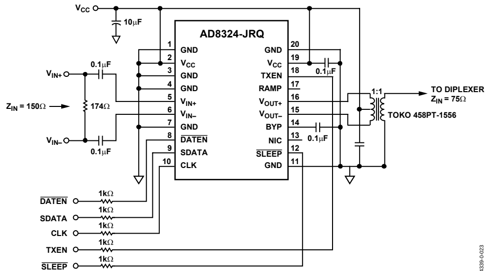
Figure 23. Typical Application Circuit
