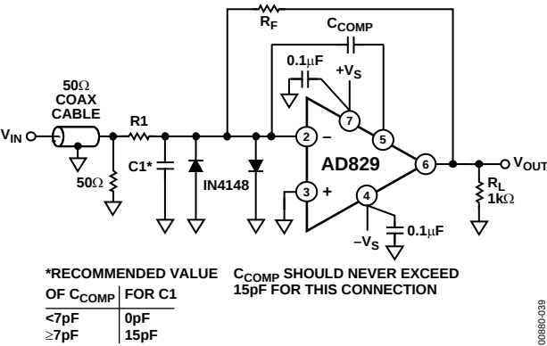
Figure 39. Inverting Amplifier Connection Using Current Feedback Compensation
