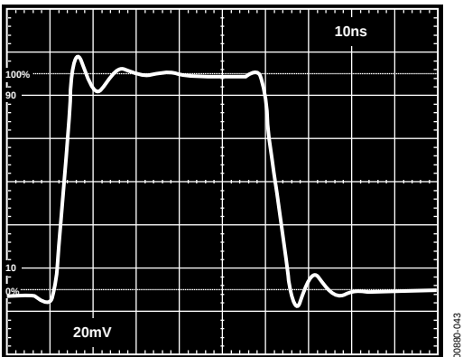
Figure 43. Small Signal Pulse Response of Inverting Amplified Using Current Feedback Compensation, C_{COMP} = 4 pF, R_F = 1 k \Omega , R1 = 1 k \Omega
