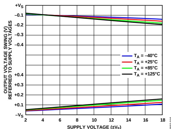
Figure 19. Output Voltage Swing (V) Referred to Supply Voltages vs. Supply Voltage Per Channel and Temperature, R_L = 10k\Omega
