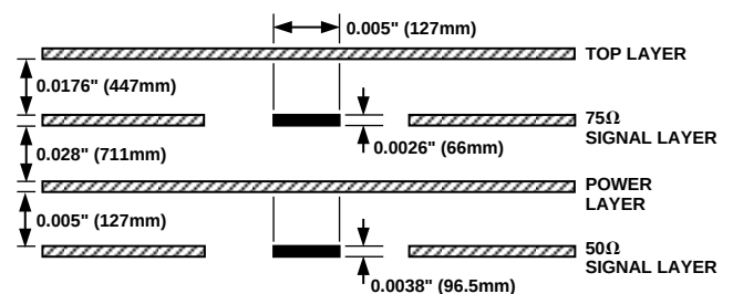
Figure 41. PCB Dimensions
