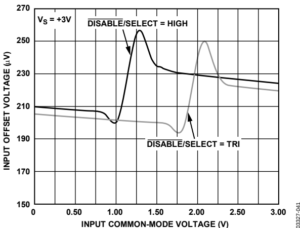
Figure 46. Input Offset Voltage vs. Input Common-Mode Voltage, V_S = 3\text{ V}
