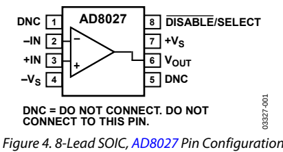
Figure 4. 8-Lead SOIC, AD8027 Pin Configuration
