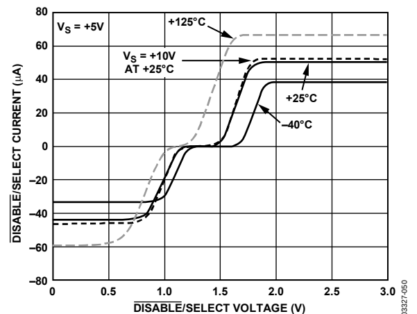
Figure 55. \overline{\text{DISABLE}}/\text{SELECT} Current vs. \overline{\text{DISABLE}}/\text{SELECT} Voltage and Temperature
