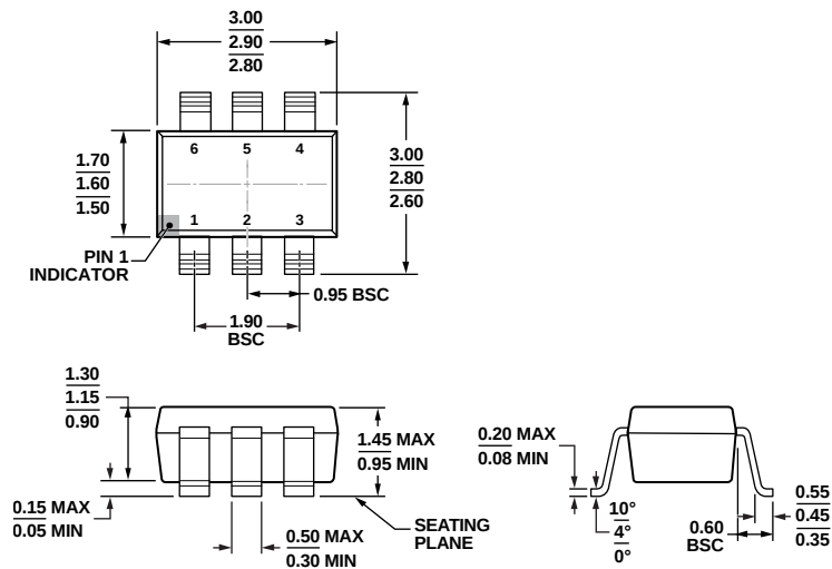
Figure 70. 6-Lead Small Outline Transistor Package [SOT-23] (RJ-6) Dimensions shown in millimeters
