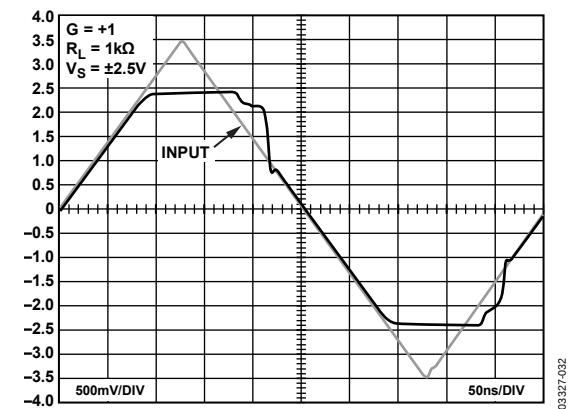
Figure 37. Overdrive Recovery, G = +1
