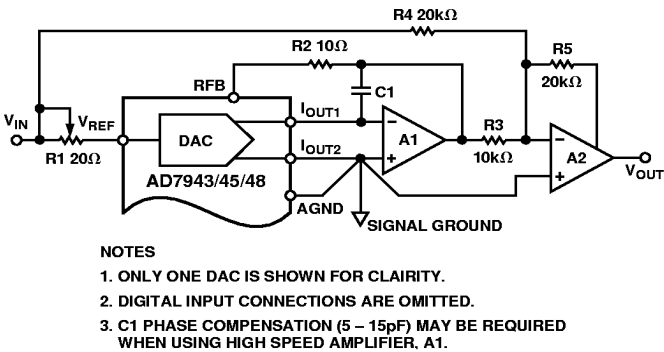
Figure 15. Bipolar Operation (Four-Quadrant Multiplication)
