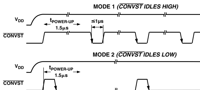
Figure 12. Power-Up Times
