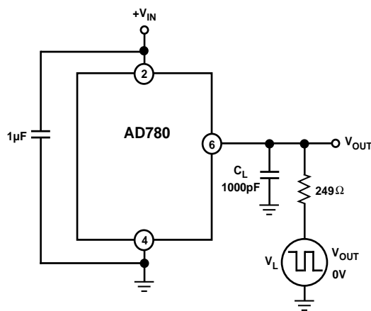
Figure 13a. Capacitive Load Transient Response Test Circuit
