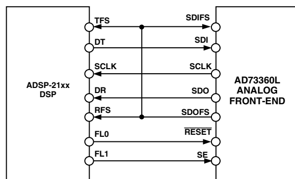
Figure 13. AD73360L Connected to ADSP-21xx
