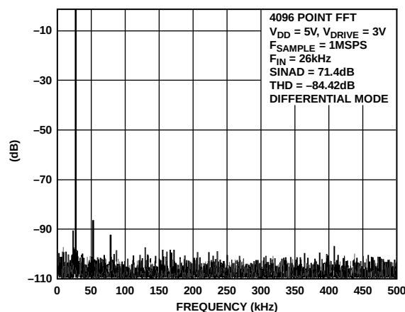
Figure 7. FFT
