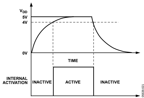
Figure 21. On-Chip Power Supply Monitor
