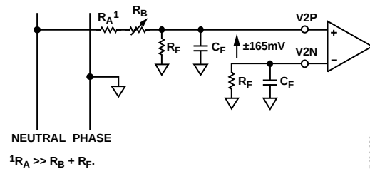
Figure 20. Typical Connections for Channel V2
