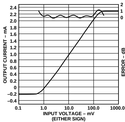
Figure 7. DC Logarithmic Transfer Function and Error Curve for Single AD641
