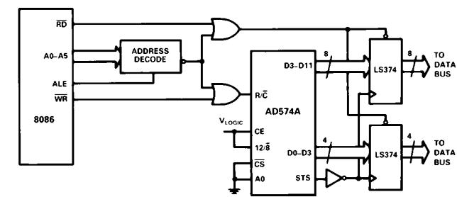
Figure 13. 8086 Stand-Alone Configuration
