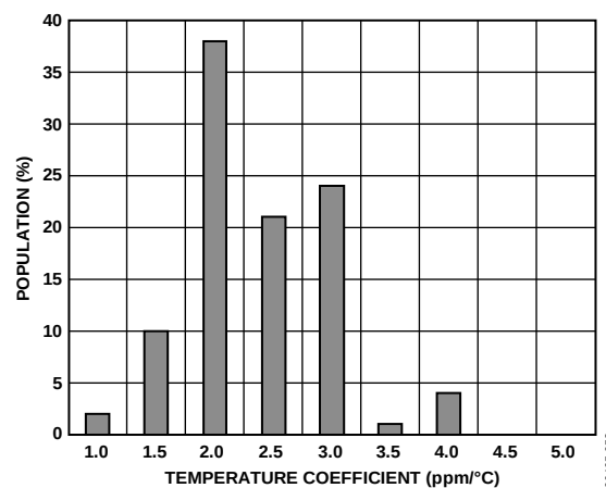
Figure 41. Reference Output TC ( 0^{\circ}\text{C} to 85^{\circ}\text{C} )
