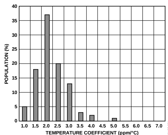
Figure 40. Reference Output TC ( -40^{\circ}\text{C} to +85^{\circ}\text{C} )
