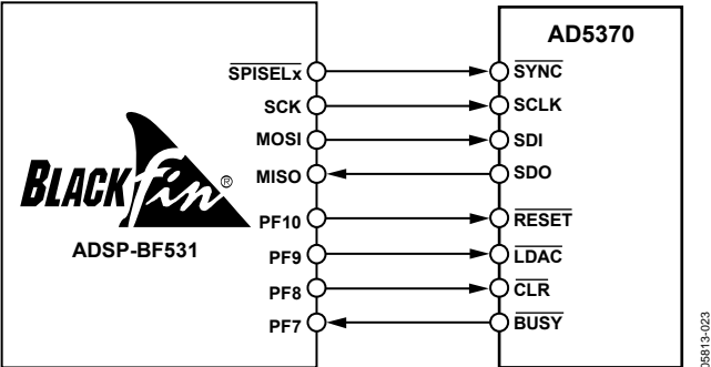
Figure 23. Interfacing to a Blackfin DSP
