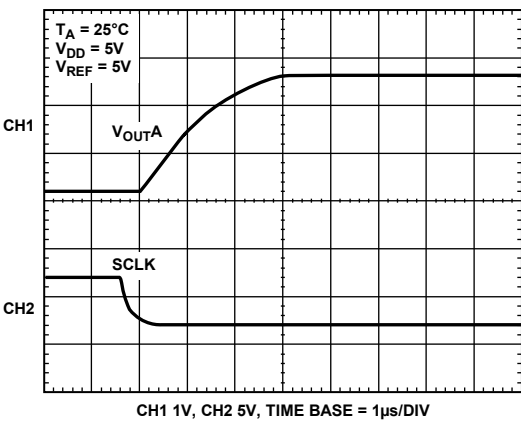
Figure 20. Half-Scale Settling ( 1/4 to 3/4 Scale Code Change)
