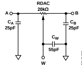
Figure 56. RDAC Circuit Simulation Model for RDAC = 20 k \Omega
