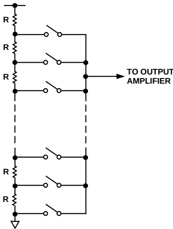
Figure 21. Resistor String
