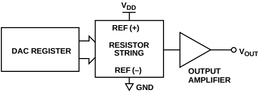
Figure 20. DAC Architecture
