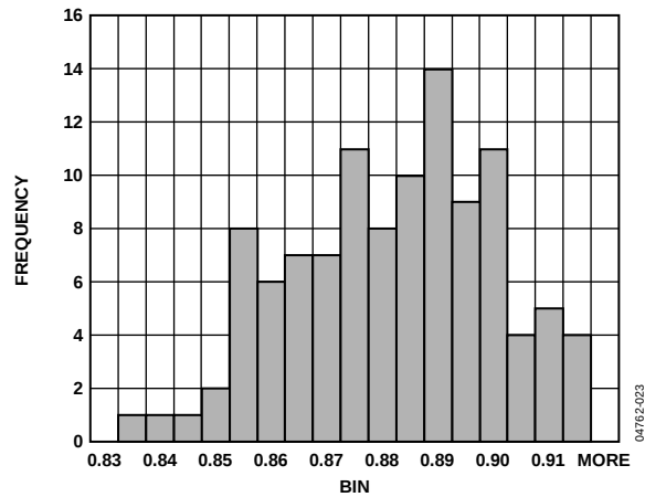
Figure 23. I_{DD} Histogram at V_{DD} = 3V
