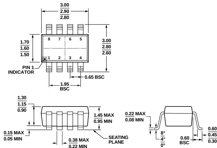
Figure 48. 8-Lead Small Outline Transistor Package [SOT-23] (RJ-8) Dimensions shown in millimeters
