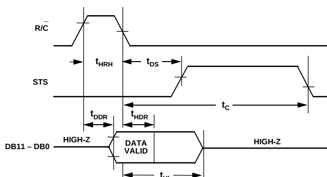
Figure 4b. Stand-Alone Mode Timing High Pulse for R/\bar{C}
