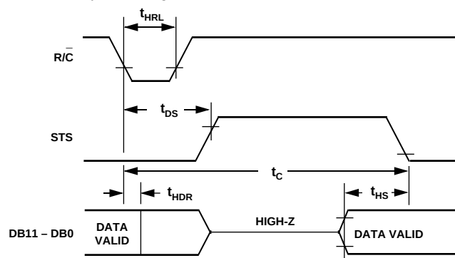
Figure 4a. Stand-Alone Mode Timing Low Pulse for R/\bar{C}
