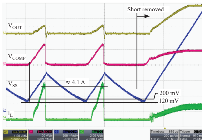
Figure 6: Hiccup Mode Operation and Recovery
