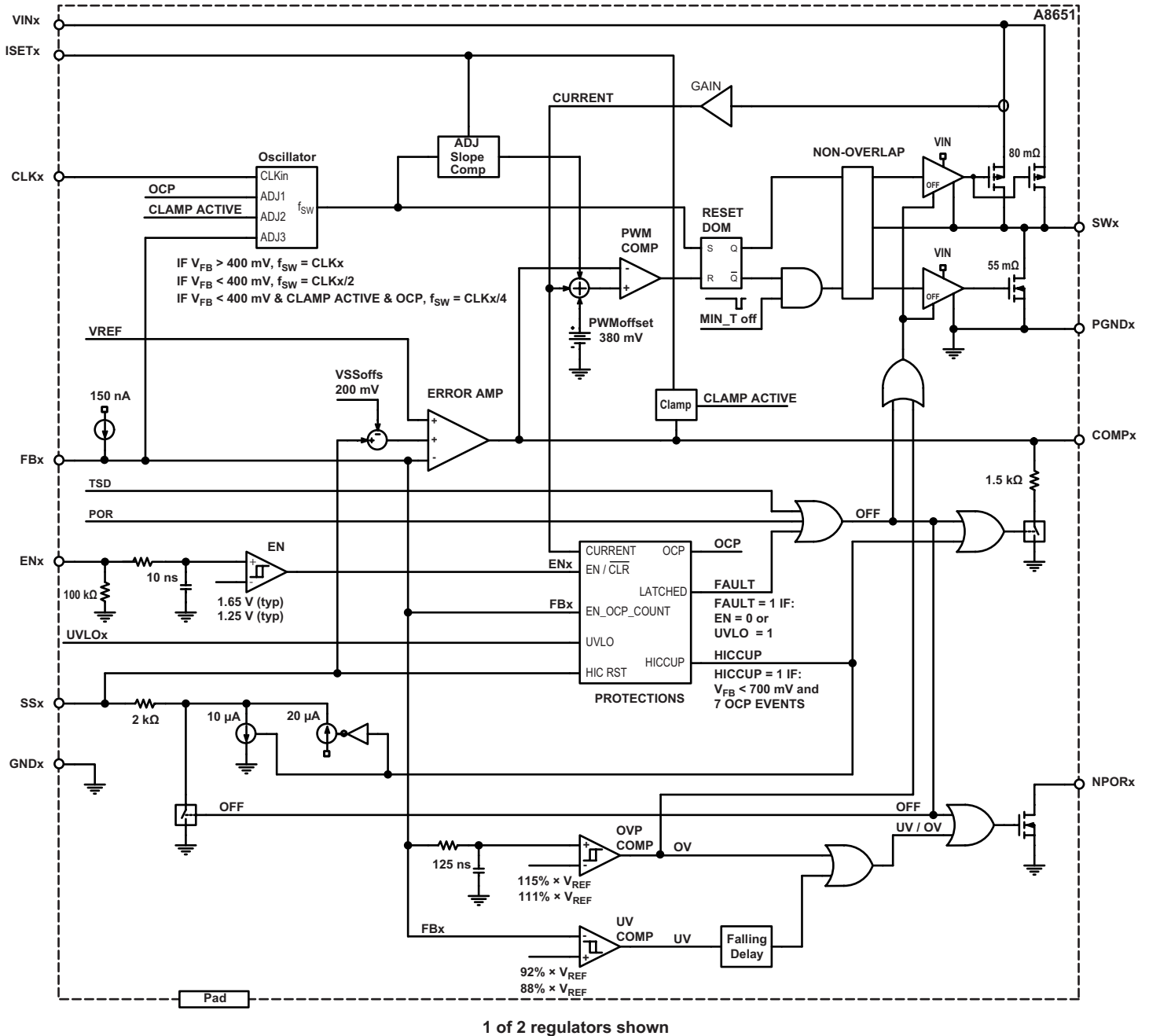
Detailed Functional Block Diagram
