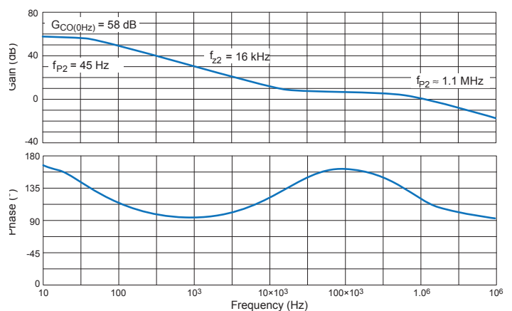
Figure 12: Type-II Compensated Error Amplifier Bode Plot
