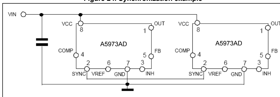
Figure 24. Synchronization example
