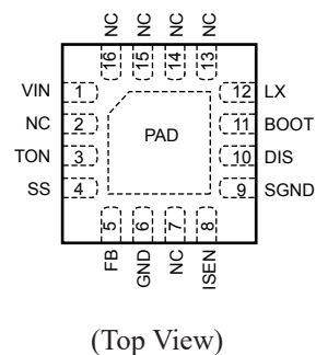
PIN-OUT DIAGRAM
