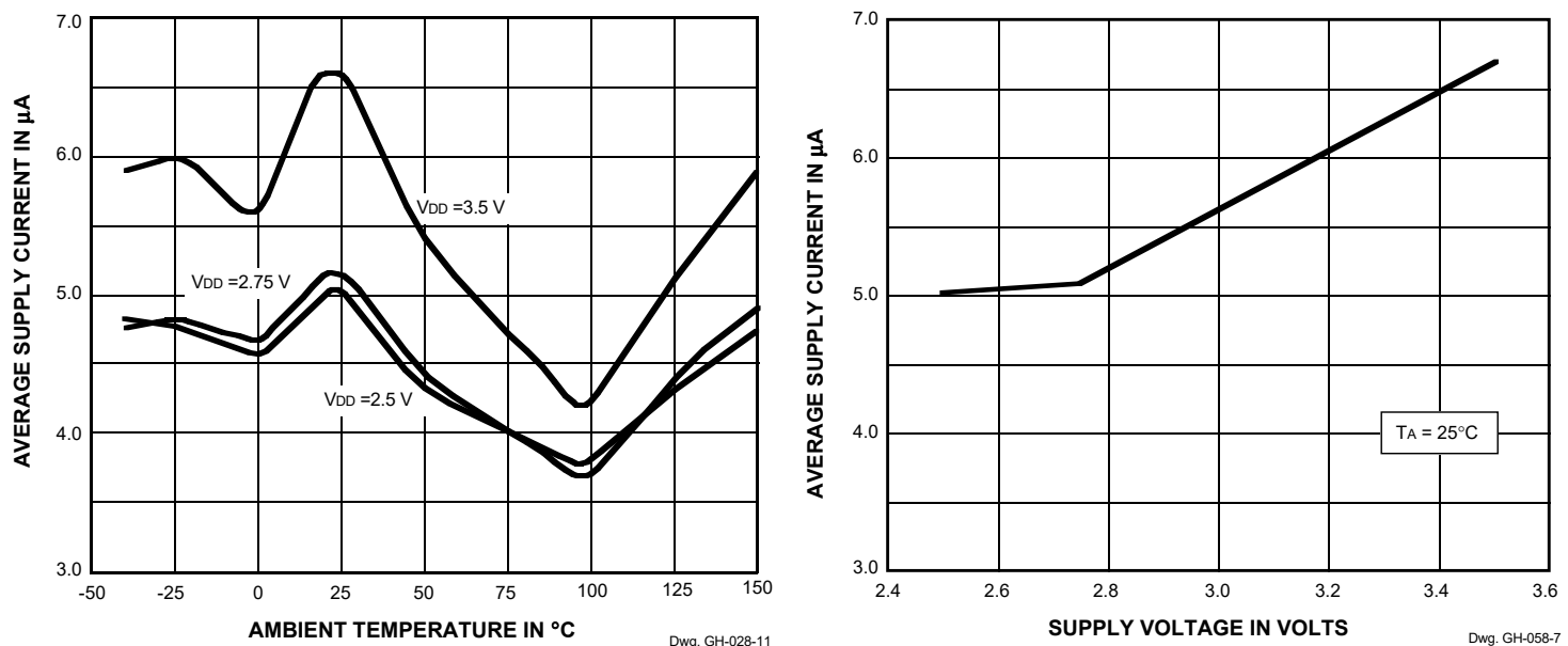
Supply Current
