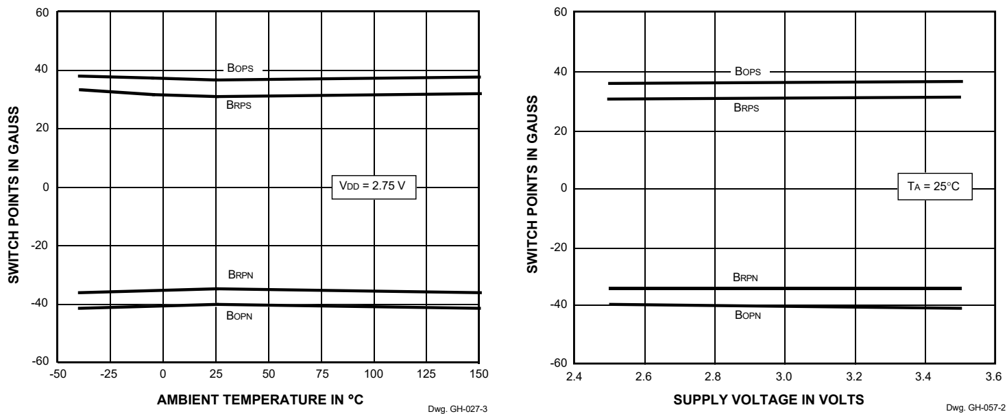
Switch Points
