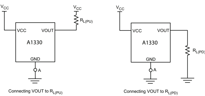
Figure 15: Connection for Detecting Broken Ground Wire
