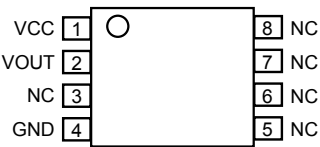
LE-8 Package Pinout (single die)
