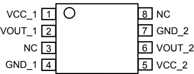
LE-8 Package Pinout (dual die)
