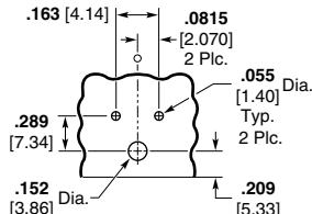
2 Circuit, In-Line
