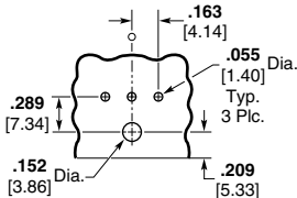
3 Circuit, In-Line
