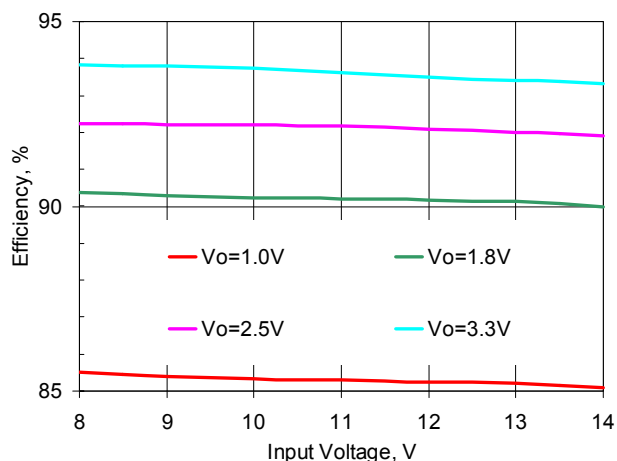
Figure 5. Efficiency vs. Input Voltage. Iout=40A, Fsw=500kHz
