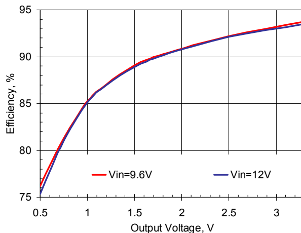
Figure 4. Efficiency vs. Output Voltage, Iout=40A, Fsw=500kHz
