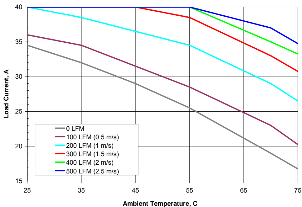
Figure 15. Thermal Derating Curves. Vin=12V, Vout=3.3V, Fsw=1MHz
