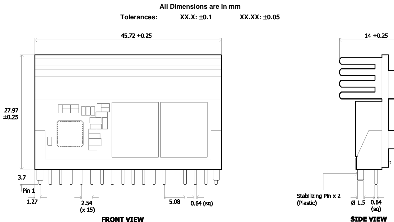
Figure 48. Mechanical Drawing
