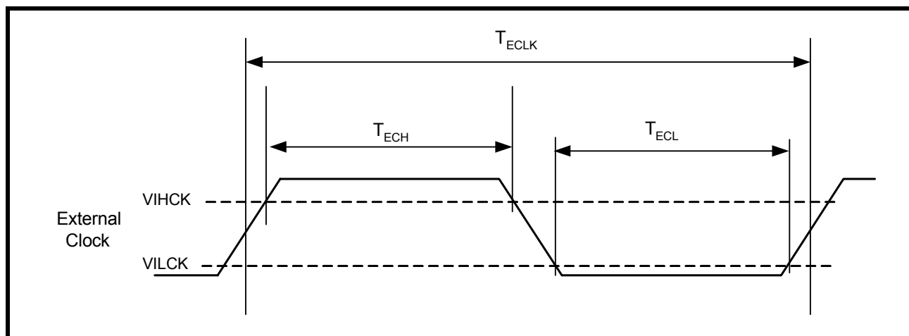
FIGURE 14. CLOCK TIMING
