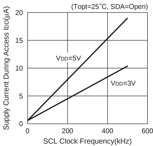
6.4 Supply Current During CPU Access vs. SCL Clock Frequency
