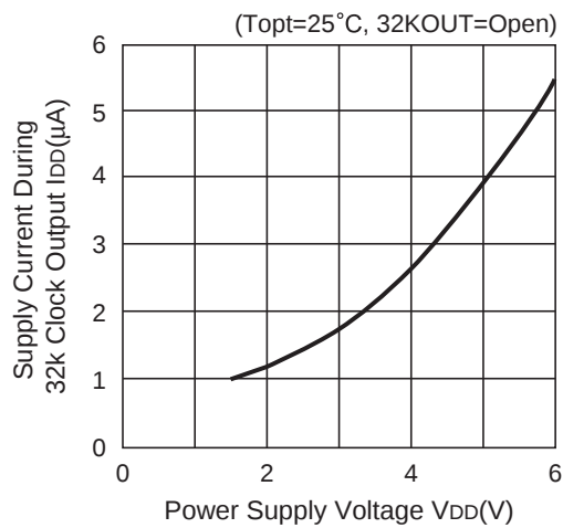
6.3 Supply Current During 32k Clock Output vs. Power Supply Voltage (RS5C372B)
