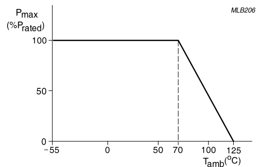
Fig. 6 Maximum dissipation ( P_{\max} ) in percentage of rated power as a function of the operating ambient temperature ( T_{\text{amb}} )
