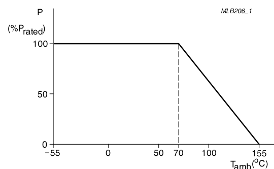
Fig. 5 Maximum dissipation ( P_{\max} ) in percentage of rated power as a function of the operating ambient temperature ( T_{\text{amb}} )
