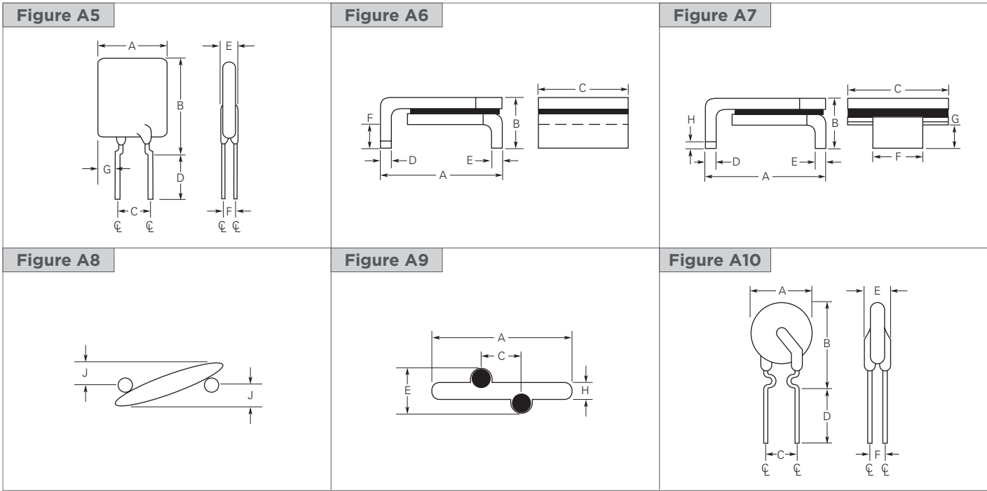
Figures A5-A13 — Dimension Figures
