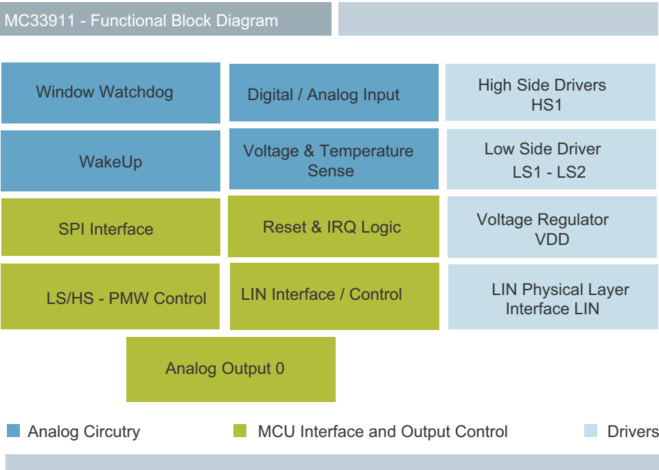
Figure 37. Functional internal block diagram
