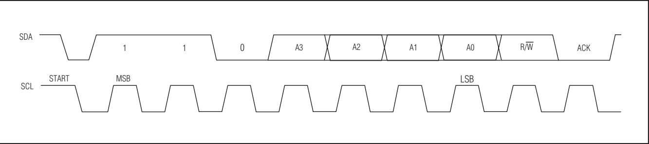
Figure 4. Slave Address
