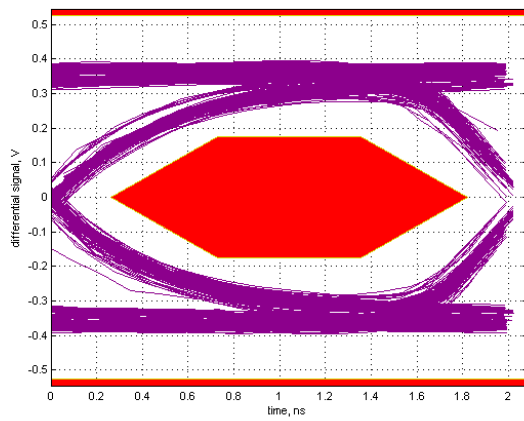
Signal Integrity USB2.0 0ohm
