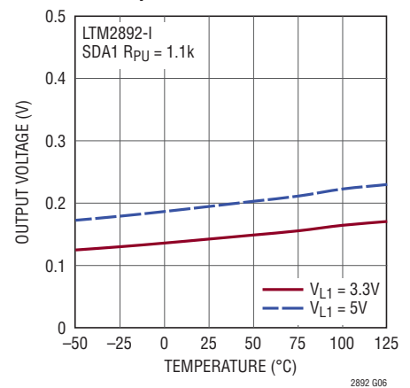
SDA1 Low Level Output Voltage vs Temperature
