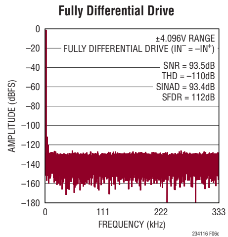
Figure 6c. IN^+/IN^- = -1\text{dBFS} 2kHz Fully Differential Sine, Common Mode = 2.5V, 32k Point FFT, f_{SAMPL} = 666\text{ksps} . Circuit Shown in Figure 6a with LT6237 Amplifiers, R_{FILT} = 24.9\Omega , C_{FILT} = 1\text{nF}
