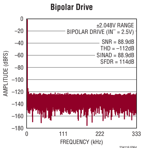
Figure 6d. IN^+ = -1\text{dBFS} 2kHz Bipolar Sine, IN^- = 2.5V , 32k Point FFT, f_{SAMPL} = 666\text{ksps} . Circuit Shown in Figure 6a with LT6237 Amplifiers, R_{FILT} = 24.9\Omega , C_{FILT} = 1\text{nF}
