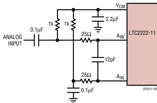
Figure 5. Single-Ended Drive
