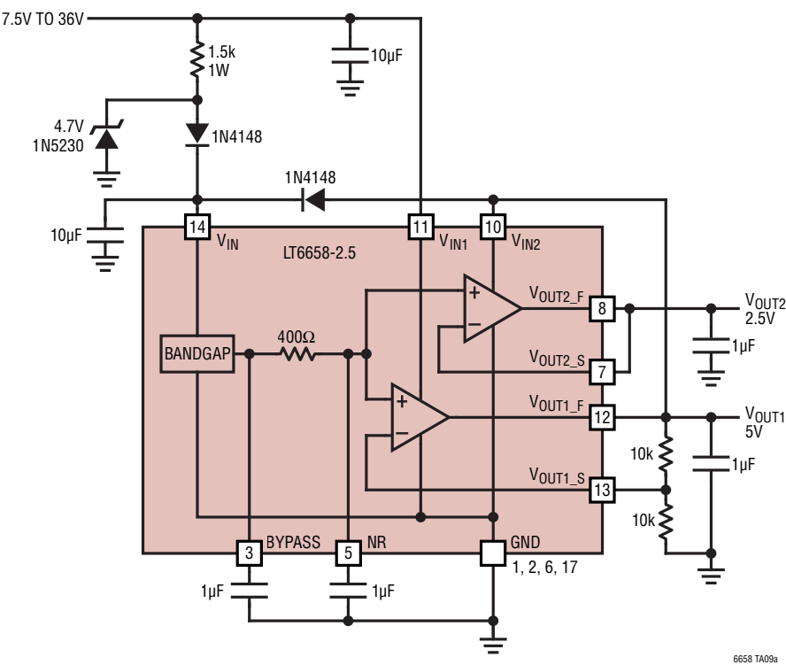
Recursive Reference Application ( V_{OUT1} Supplies Power to V_{IN} and V_{IN2} )
